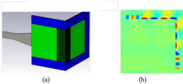
Figure 5: (a) Experimental Setup used to test a sharp corner (90-degree) waveguide; (b) 2D electric field distribution of both guided- and surface- wave along the waveguide structure under test.
