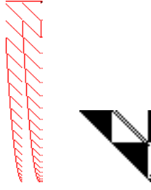
Fig. 5 Example for the sparsity pattern of the Jacobian of the constraint functions (left) and of the upper-right triangle of the Hessian of the Lagrangian function (right) for instance QPLIB_2967. The gradient of the objective function is displayed as the first row of the Jacobian matrix. Non-constant entries are shown in red.
