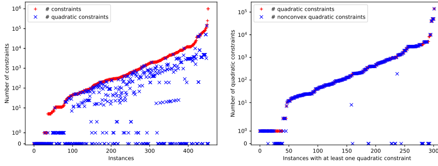
Fig. 3 Number of constraints, quadratic constraints, and nonconvex quadratic constraints of QPLIB instances.
