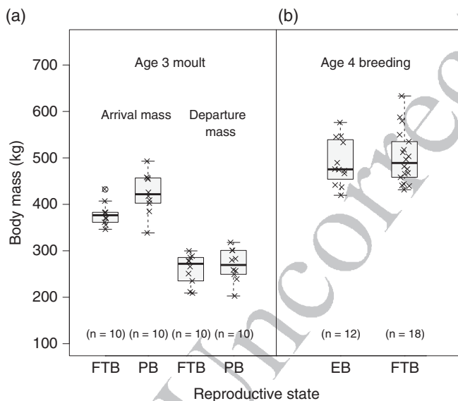
FIGURE 6 Variation in body mass as a function of reproductive state for female southern elephant seals at Marion Island. (a) The moult arrival and departure body mass of age 3 females that were first-time breeders (FTB) in the preceding breeding season is compared to the body mass of prebreeders (PB) (i.e., individuals that deferred breeding at age 3). (b) The breeding season arrival body mass of age 4 experienced breeders (EB, that is, females that were FTB at age 3) relative to age 4 females with no previous breeding experience (FTB). Horizontal boxplot lines show the median mass and boxes represent the 25th and 75th percentiles, respectively. Individual observations (x) are superimposed on boxplots
