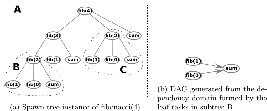
Fig. 2: Data structures related to the task-based Fibonacci example
