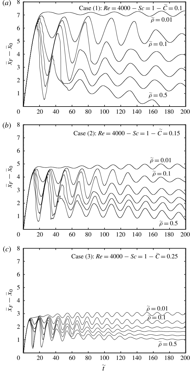
FIGURE 15. Time evolution of the front displacement \bar{x}_F - \bar{x}_0 for C = 0.1 (a), 0.15 (b), 0.25 (c), where \bar{x}_F is defined as the maximum location where the span-averaged density field at the bottom wall is \tilde{\rho} = 0.01, 0.1, 0.2, 0.3, 0.4 and 0.5 , respectively.
