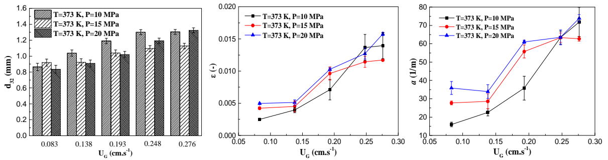
Fig. 4 Bubble mean Sauter diameter (left), gas holdup (middle) and interfacial area (right) under various superficial gas velocity and pressure at T=373K and U_L = 0.022\text{cm.s}^{-1}
