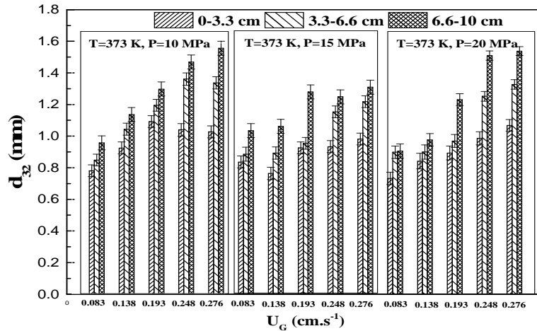
Fig. 5 Bubble mean Sauter diameter along the location of the column under various superficial gas velocity and pressure at T=373K and U_L = 0.022\text{cm.s}^{-1}
