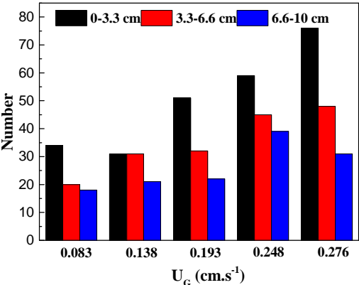
Fig. 6 Bubble number distribution along the location of the column under various superficial gas velocity at T=373K and P=10MPa
