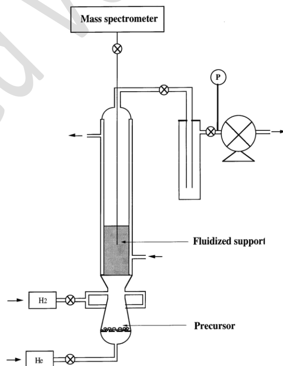
Figure 4 Schematic diagram of the fluidized-bed CVD reactor.
