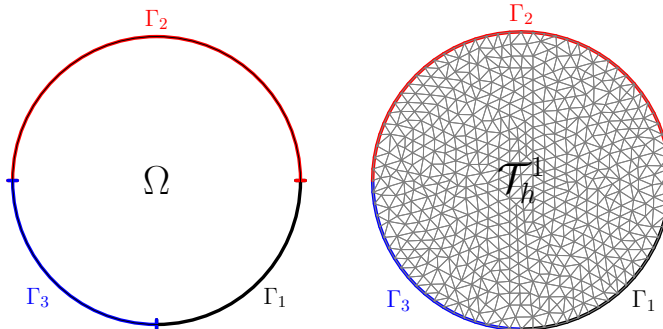
Figure 1: Unit disk \Omega with the partition of its boundary (left) and the associated mesh \mathcal{T}_h^1 (right).
