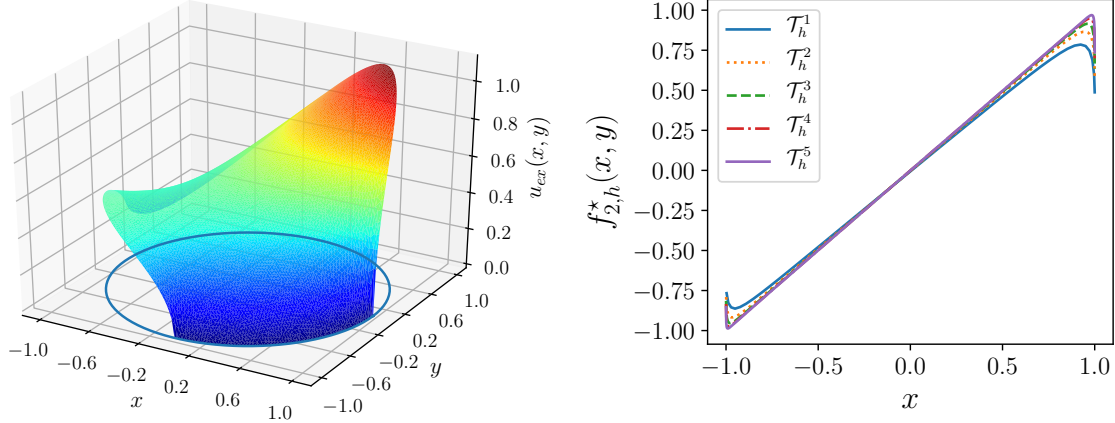
Figure 2: Optimal solution u_h^* (left) on \mathcal{T}_h^3 and the optimal control f_{2,h}^* computed on different meshes for \rho = 10 and data from Experiment 2.
