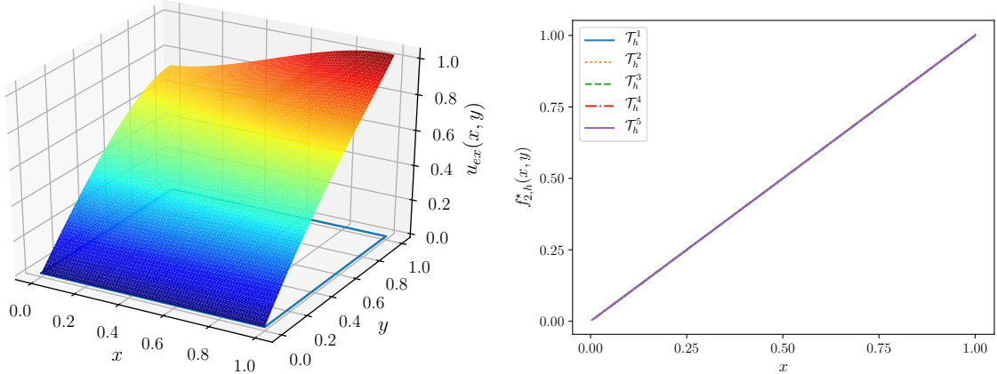
Figure 3: Optimal solution u_h^* (left) on \mathcal{T}_{s,h}^3 and the optimal control f_{2,h}^* computed on different meshes for \rho = 10 and data from Experiment 2.
