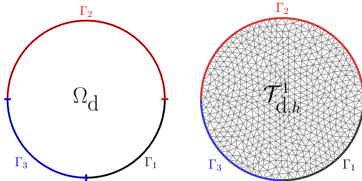
Figure 1: Unit disk \Omega_d with the partition of its boundary (left) and the associated mesh \mathcal{T}_{d,h}^1 (right).
