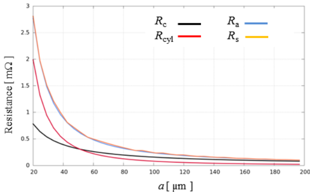
Figure 2 - Resistance of an a-spot as a function of its radius a : 2D-axisymmetric simulations ( R_s ) and Holm's theory ( R_c )
