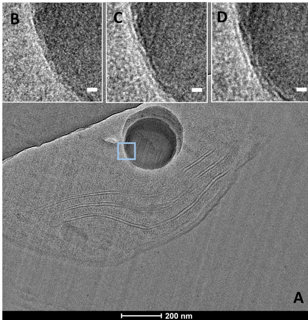
FIGURE 7 | CEMOVIS images of G. lithophora . (A) Image a cell with one ACC inclusion. (B–D) Close-ups of the ACC inclusion (see outline in A ), showing a membrane/shell around the inclusion (white arrows). Images were acquired at several focus heights: (B) -1\ \mu\text{m} , (C) -2\ \mu\text{m} , and (D) -3\ \mu\text{m} . Scale bars: (B–D) 10 nm.
