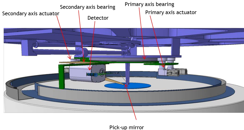
Figure 11. The Low-order wavefront sensor within its theta-phi navigation stage.
