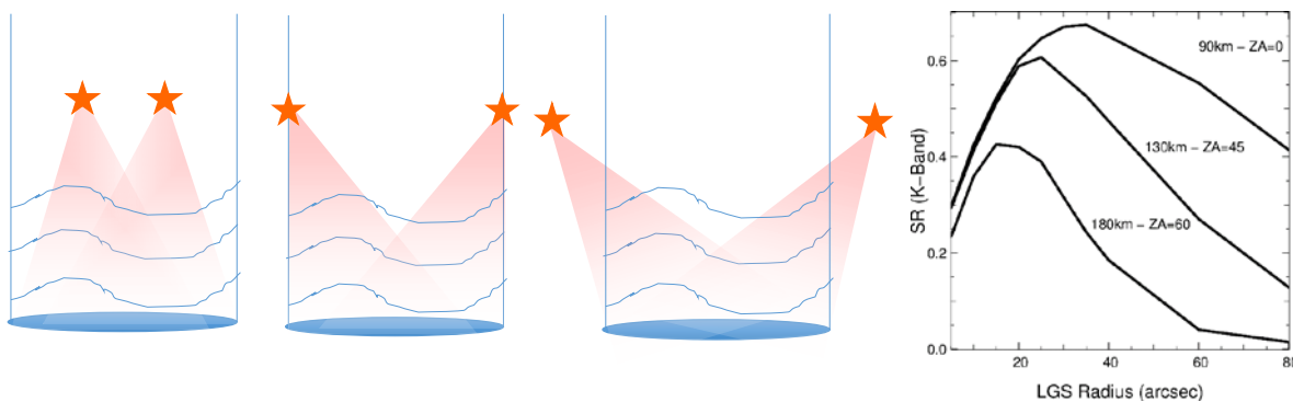
Figure 7. Left: Illustration of various asterism radii. The second cartoon corresponds to optimal asterism. Right: Strehl ratio as function of LGS asterism radius for three different Zenith angles (ZA).
