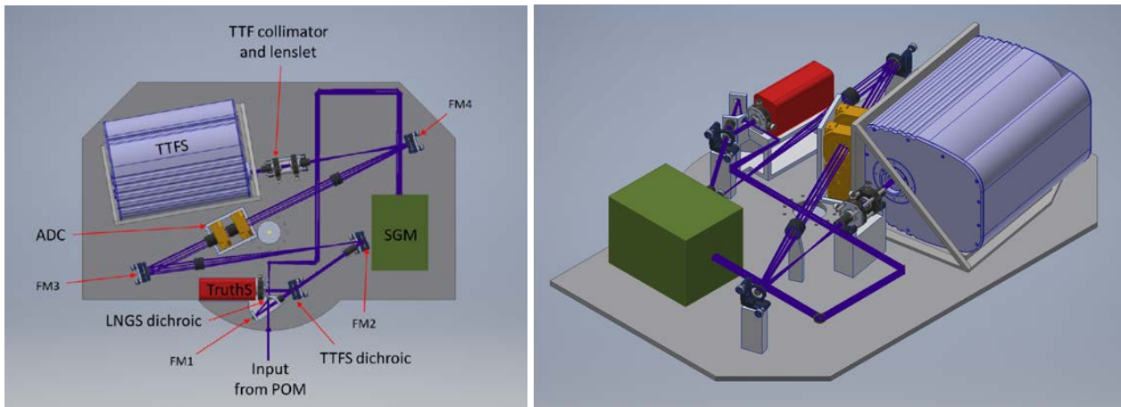
Figure 10. Preliminary mechanical layout of LGNS sensors.
