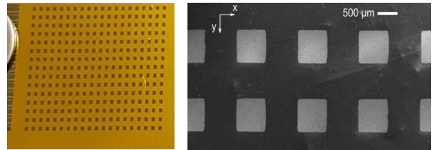
Fig. 3. (a) Photograph of the printed MIM metasurface, and (b) SEM image of the printed structure
