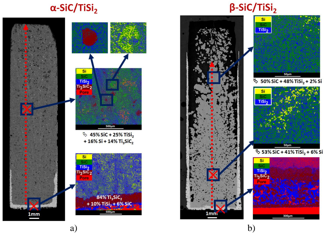
Figure 9. Optical and colored backscattered electrons images of the cross sections of the SiC compacts infiltrated by molten TiSi 2 at 1550°C for 1h: a) α-SiC and β-SiC. The local surface fractions are given for whole image surface with an accuracy of ±5%.
