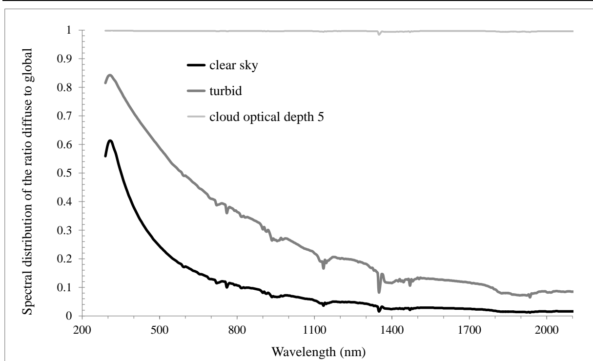
Figure 6.11. Ratio of the diffuse irradiance to the global irradiance as a function of wavelength for a solar zenithal angle of 30^\circ and two cases of cloud-free conditions: clear sky (visibility of 50 km) and turbid (visibility of 10 km) as well as a cloudy situation with an optical depth of 5.
