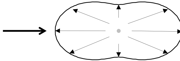
Figure 6.1. Schematic scattering patterns in the case where particles or molecules are much smaller than the incident wavelength. The thick black arrow denotes the incident light. The further the limit of the pattern from the particle or molecule (in grey), the greater the probability the light may be scattered in that direction.
