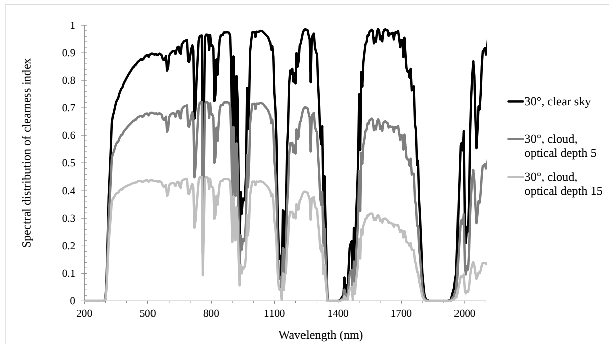
Figure 6.8. Typical spectral distribution of clearness index for wavelengths from 200 nm to 2000 nm for a solar zenithal angle of 30^\circ . The surface is horizontal at ground level. Clear sky conditions (visibility of 50 km, black line) and cloudy conditions with two optical depths: 5 (dark grey line) and 15 (light grey line).
