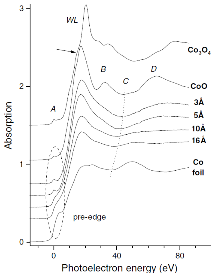
Figure 3. XANES spectra obtained at the Co K-edge of the as-deposited Co/ZrO 2 (CEY—300 K) DML grown at a deposition rate of 0.5 \text{ \AA s}^{-1} , compared with those of metallic Co foil, CoO and Co 3 O 4 . Spectra are shifted for clarity.
