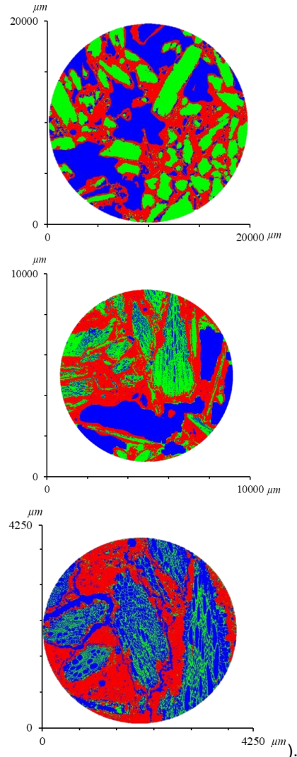
Figure 4 - X-ray tomography slice of MS concrete (voxel size of 4 \mu\text{m} )
