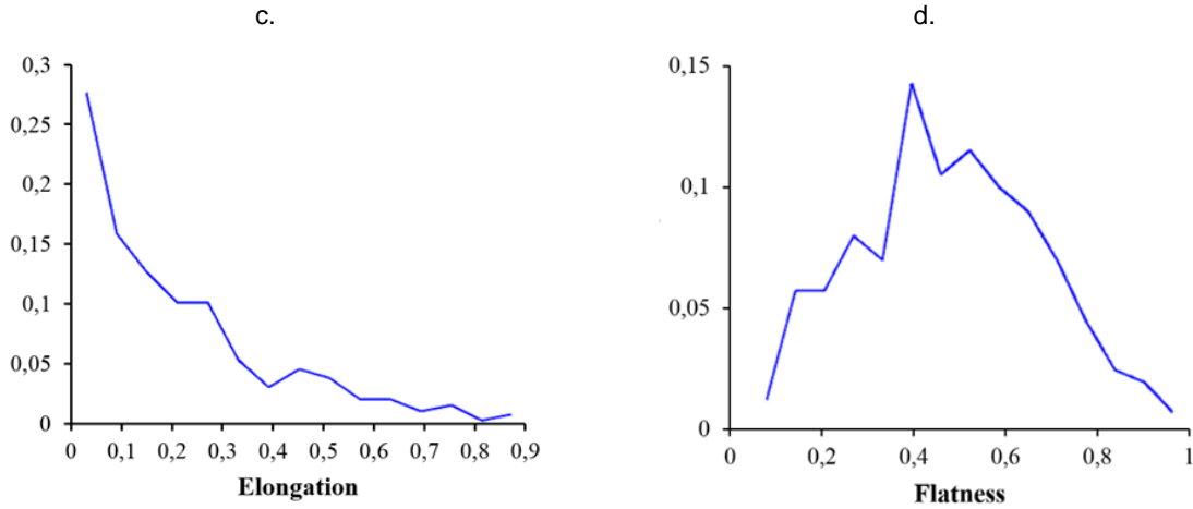
Figure 7 – 399 particles sunflower bark chips are each assimilated to a stress ellipsoid (a) and three shape parameters are calculated and presented as normalized histograms, namely (b) anisotropy, (c) elongation, and (d) flatness.
