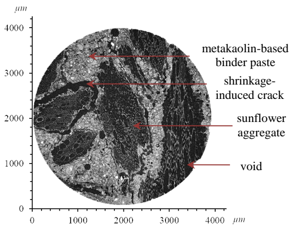
Figure 4 - X-ray tomography slice of MS concrete (voxel size of 4 \mu\text{m} )
