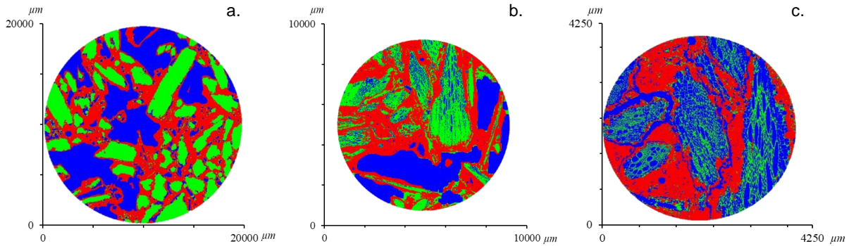
Figure 5 - Identification of binder (red), aggregate (green) and void (blue) phases in MS composite for three different scan resolutions with voxel sizes of (a) 19.9 \mu\text{m} , (b) 10 \mu\text{m} and (c) 4 \mu\text{m}
