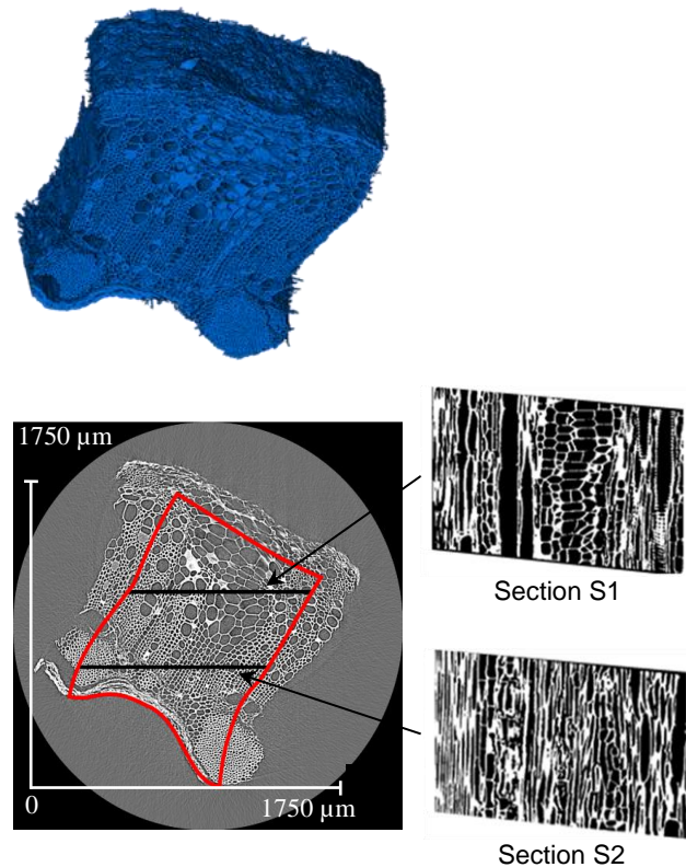
Figure 3 – (a) 3D tomographic reconstruction of a sunflower bark chip, and (b) cross-section through the 3D volume.
