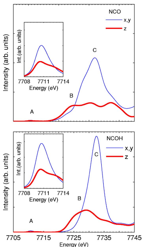
FIG. 5. (Color online) Calculated Co K -edge XAS spectra in NCO (upper graph) and NCOH (lower graph) for the two polarization directions, in plane (thin lines) and out of plane (thick lines). The preedge region is enlarged in the insets.
