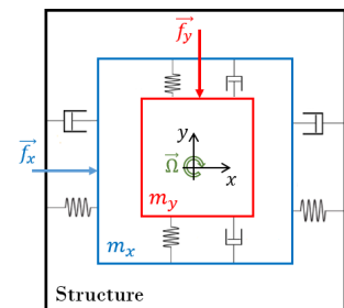
Fig. 1. MEMS gyroscope scheme.
