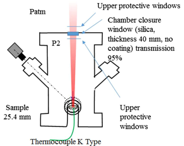
FIG. 1. Pressure vessel for experiments with a pressurized gaseous oxygen atmosphere.
