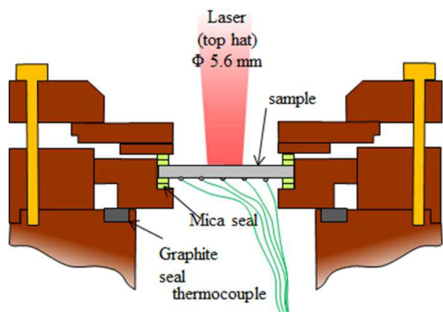
FIG. 2. Geometry of the sample holder.
