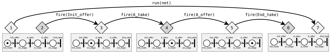
(a) Target Petri net execution trace. This execution is hidden from runtime services connected to the activity diagram execution.
