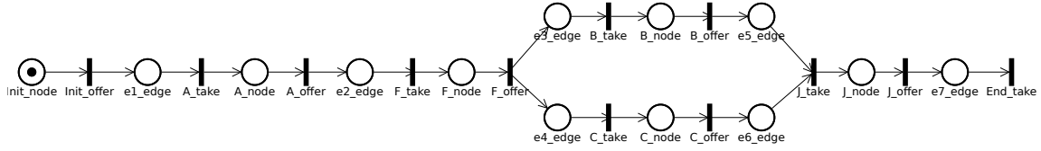
Figure 5: Petri net produced by the compilation of the activity from Figure 4, conforming to the interpreted DSL from Figure 1.
