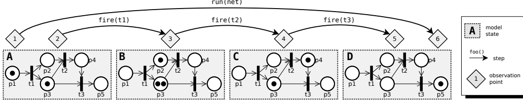
Figure 2: Example of execution trace of a Petri net model conforming to the Petri net DSL shown in Figure 1.
