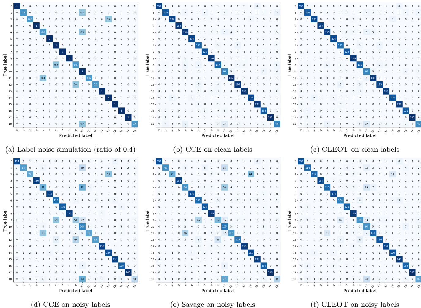
Fig. 4: Confusion matrix of different methods on NWPU19. First row indicates the confusion matrix with the clean labels and second row with noisy labels. The class names are in the following order (starting index from ‘0’): airplane, baseball diamond, beach, chaparral, dense residential, forest, freeway, golf course, harbor, intersection, medium residential, mobile homepark, overpass, parking lot, river, runway, sparse residential, storage tanks, tennis court.
