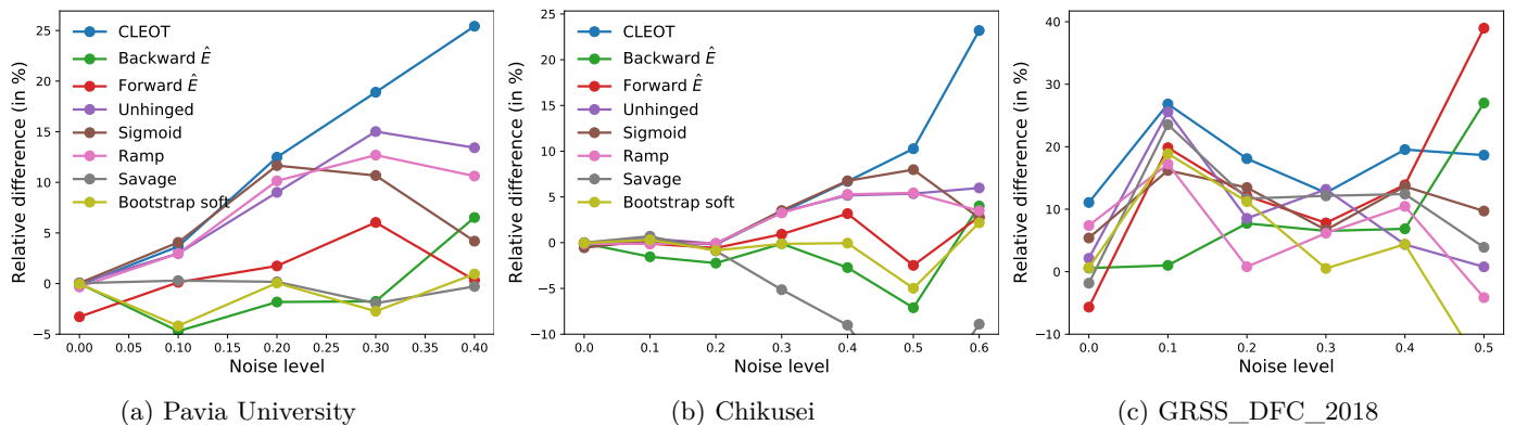
Fig. 3: Relative difference in performance of our proposed method and state-of-the-art methods with respect to cross entropy loss function for the three hyperspectral datasets: (a) Pavia University, (b) Chikusei, (c) GRSS_DFC_2018.
