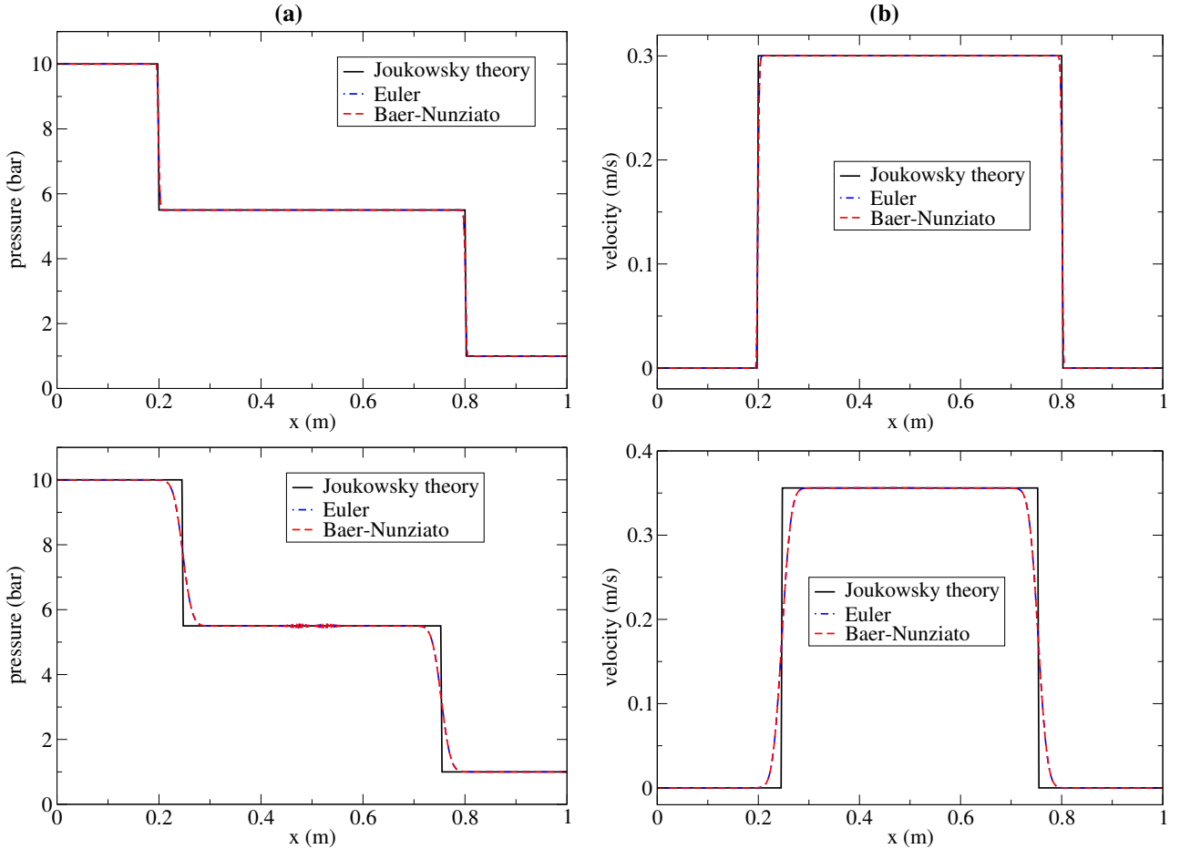
Figure 12: Test 6: Comparison between numerical and Joukowsky-type solutions on the Riemann problem in rigid (top) and elastic (bottom) pipes at t = 2 \times 10^{-4} s with 800 cells: (a) mean pressure p = \alpha_1 p_1 + \alpha_2 p_2 and (b) phasic velocity u_1 .
