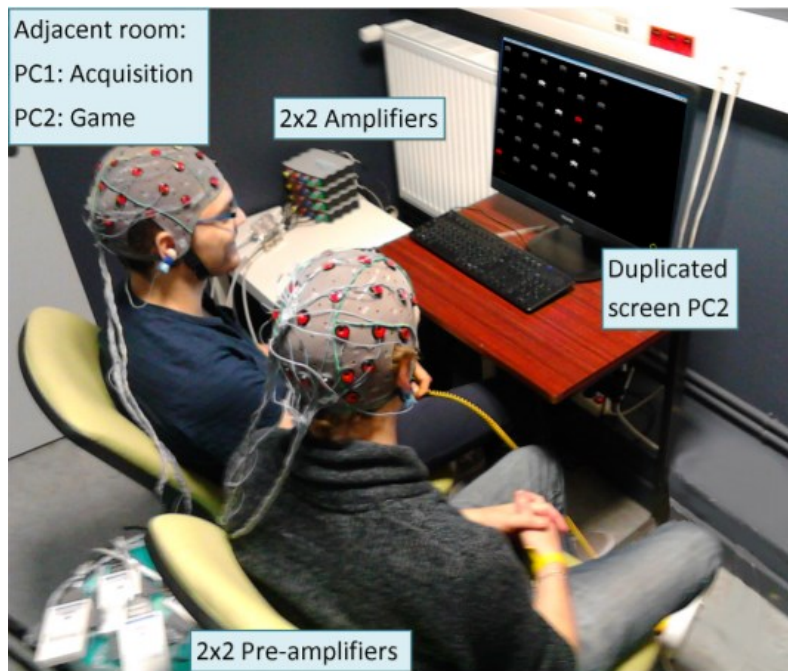
Figure 2. Experimental setup.
