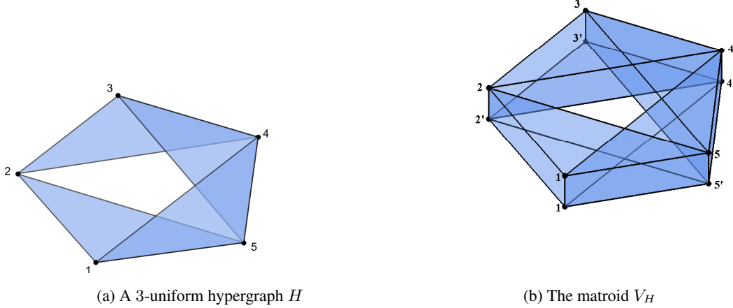
(a) A 3-uniform hypergraph H
