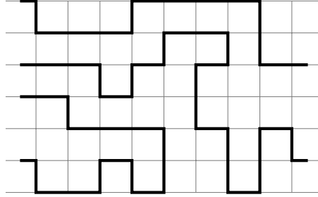
Fig. 2: A 9-block of the 6 \times 0 tube. This 9-block has length 50.
