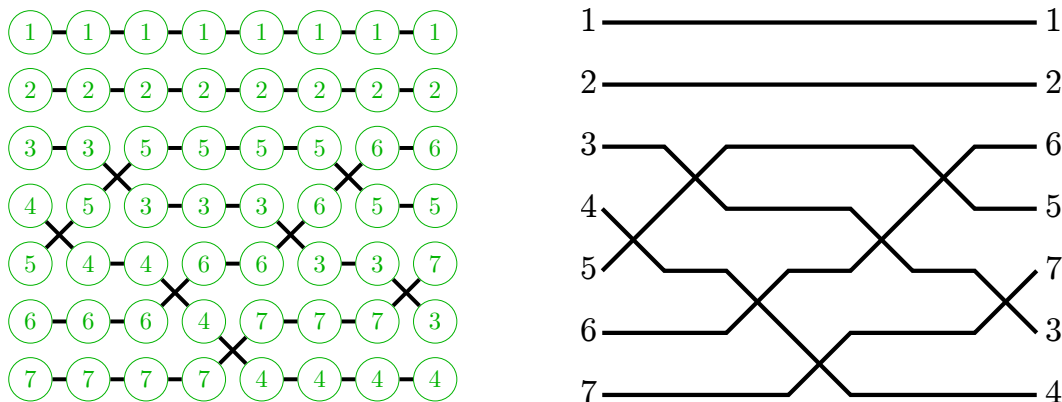
Fig. 2: The wiring diagram for the reduced word (4, 3, 5, 6, 4, 3, 5) \in R([1, 2, 6, 5, 7, 3, 4]) showing the intermediate permutations on the left and a simplified version of the same wiring diagram on the right. The crossings in positions 2 and 6 are both in row 3.
