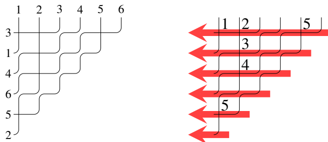
Fig. 4: A reduced pipe dream for w = [3, 1, 4, 6, 5, 2] . The corresponding reduced word is \mathbf{a} = (5, 2, 1, 3, 4, 5) and x^D = x_1^3 x_2 x_3 x_5 .
