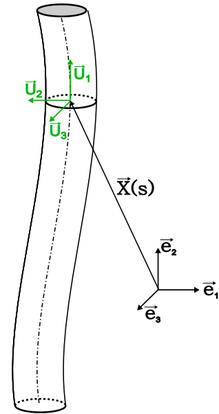
Fig. 8. Yarn geometry.
