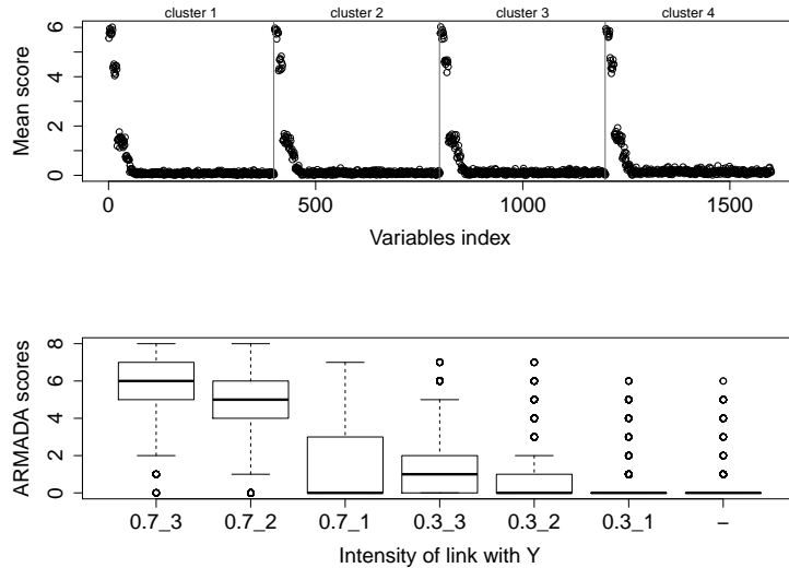
Figure A2. Top: mean of the ARMADA scores obtained by all the covariates. Bottom: boxplot of the scores of the covariates, ranked by levels of link with Y . Means and boxplots are calculated on N = 100 runs. Simulation in the classification design.
