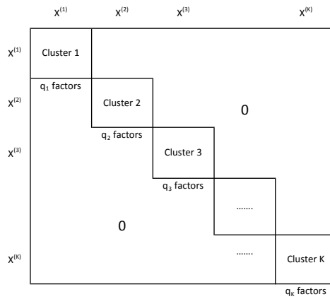
Figure 1. Covariance structure of covariates given Y
