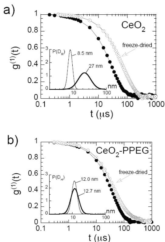
Figure 9. Re-dispersion in aqueous solutions of CeO_2 and PPEG- CeO_2 powders obtained by freeze-drying both stock solutions. a) Correlation functions of the original sol before and after freeze-drying and re-dispersion. The inset shows the derived hydrodynamic radii D_H distribution. a) id. hybrid sol. For sake of comparison, the diffusion coefficients have been measured at a concentration of 0.1%. They have not been extrapolated to zero concentration leading to slightly smaller D_H than in Table 1.
