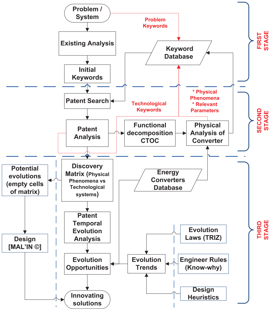
Figure 2. Block diagram of proposed method. Dotted line arrows indicate the entrances to the keyword database. Dashed line arrows indicate the divisions between stages.
