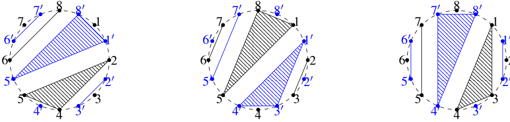
Fig. 4: Applying the Kreweras complement \kappa to the noncrossing partition \pi = \{(2, 4), (4, 5), (6, 8)\} shown at left yields \kappa(\pi) = \{(1, 5), (2, 3), (5, 8), (6, 7)\} , which is the blue noncrossing partition on the left, and the black one in the middle. Applying \kappa twice yields \kappa^2(\pi) = \{(1, 3), (3, 4), (5, 7)\} , shown at right. The convex hulls of \kappa^2(\pi) and \pi differ by a counterclockwise rotation of 2\pi/8 radians.
