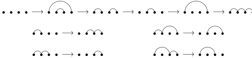
Fig. 3: The five orbits of w = \tau_{3,4}\tau_{1,2}\tau_{2,3}\tau_{1,4} on \text{NC}(4) . Notice that in any orbit, the average of the arc count is \frac{3}{2} .
