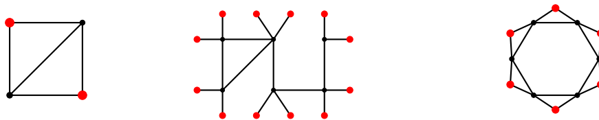
Fig. 5: Three example constructions of 2-cliquish graphs. The maximal independent sets are the large red vertices.
