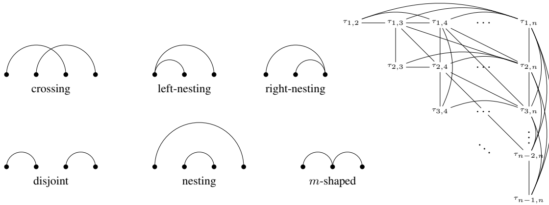
Fig. 2: Top left: the three disallowed pairs of arcs in a noncrossing partition, also the three noncommuting pairs of toggles. Bottom left: the three commuting pairs of toggles. Right: The base-graph \Gamma_n of the toggle group W_n .
