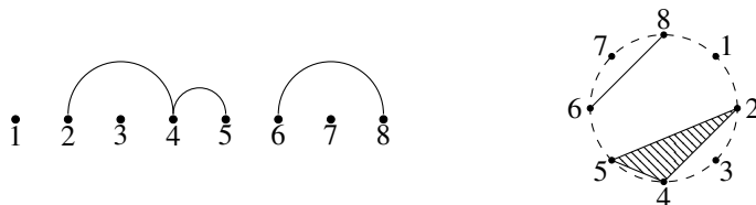
Fig. 1: The linear representation P = \{(2, 4), (4, 5), (6, 8)\} of the noncrossing partition \pi = \{\{1\}, \{2, 4, 5\}, \{3\}, \{6, 8\}, \{7\}\} at left, and the circular representation on the right.
