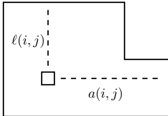
Fig. 1: Arm and leg length of boxes in Young diagrams.
