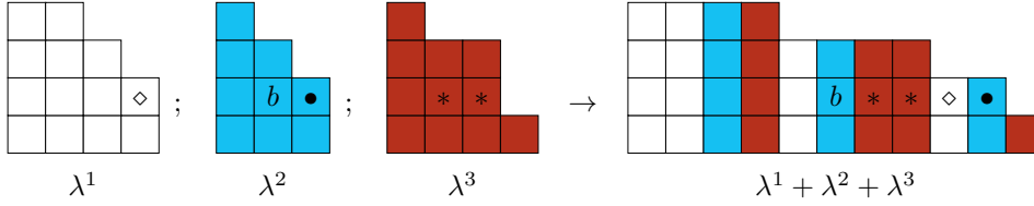
Fig. 2: The diagram of an entry-wise sum of partitions.
