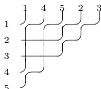
Fig. 5: The bottom reduced pipe dream for [14523] obtained by aligning the diagram to the left.
