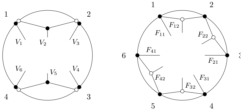
Fig. 3: The diagram on the left indicates schematically how to produce a tensor diagram for \text{Conf}_4(\text{SL}_3) from a tensor diagram for \text{Gr}(3, 6) . This is done by plugging in the vectors V_1, \dots, V_6 to the black strands in the figure. The right figure indicates how to produce a tensor diagram for \text{Gr}(3, 6) from a tensor diagram for \text{Conf}_4(\text{SL}_3) . The arguments F_{11} and F_{12} indicate the black and white parts of the first affine flag and so on.
