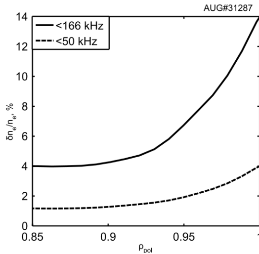
Figure 4. Density fluctuation level for frequencies f < 166 kHz (solid) and f < 50 kHz (dashed) in the ELM-free phase of the H-mode with ECMs, t = 2.141 s
