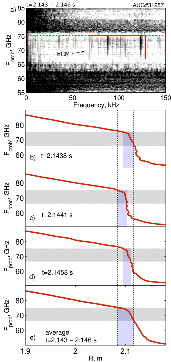
Figure 2. (a) Frequency spectra for all probing frequencies during the I-phase AUG#31287. The ECMs are measured with probing frequencies of 67–75 GHz within the time window t = 2.143\text{--}2.146 \text{ s} of typical FFT, corresponding to the region from the strong gradient localisation to the top of the pedestal. Absolute position of UFSR measurement for different probing frequencies is shown in (b–e), as individual profiles (b–d) and in average over 3 ms (e). Blue rectangles demonstrate how the probing frequency range can be interpreted in terms of radial position (b–d) and create an additional broadening of the mode localisation (e)
