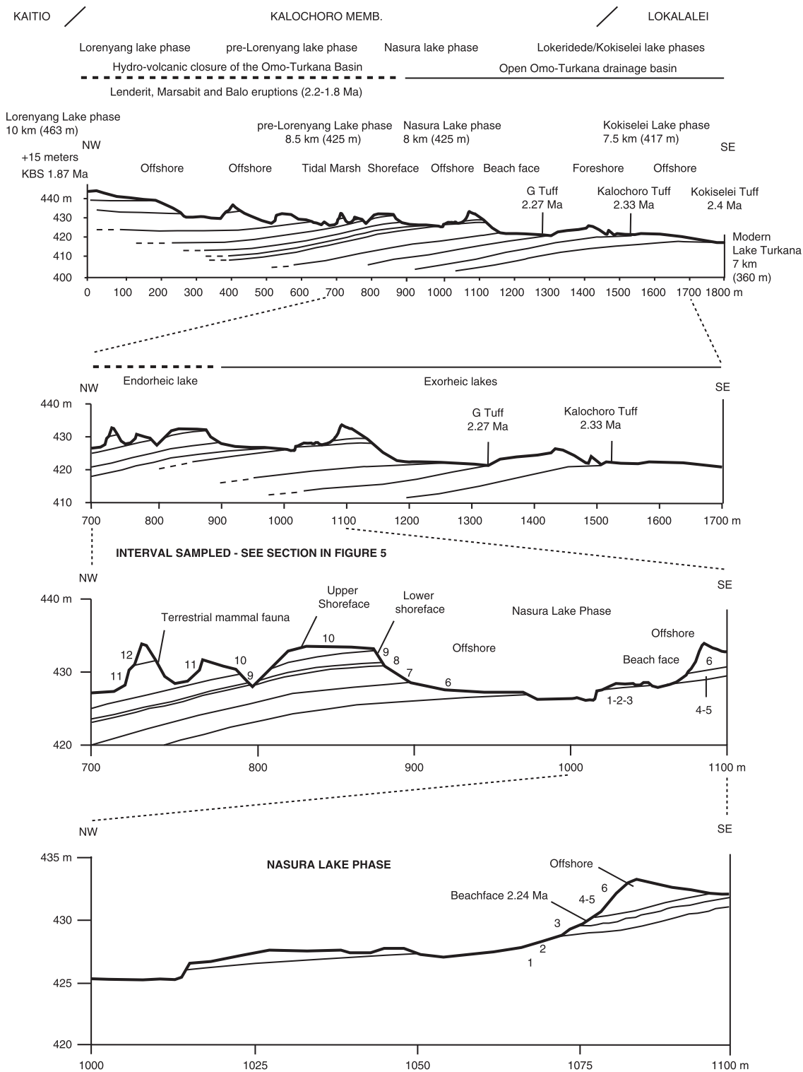
Figure 2. Geologic cross sections with the location of the studied paleolakes and volcanic tuffs. The 2.33 \pm 0.02 Ma Kalochoro Tuff delimits the transition between the Lokalalei and Kalochoro Members. The 1.87 \pm 0.02 Ma KBS Tuff delimits the Kalochoro and Kaitio boundary. Distances to modern Lake Turkana are reported for each paleolake phase. Numbers denote lithostratigraphic units described in Figure 5.
