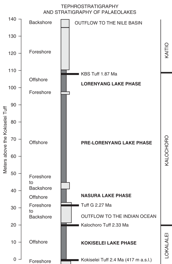
Figure 3. Stratigraphic column of the upper Lokalalei, Kalochoro, and lower Kaitio Members, linking the lacustrine sediments (offshore clays to foreshore sands) with the volcanic tuffs locally identified within these geologic members (see the identified volcanic tuffs presented in the Table 1).
