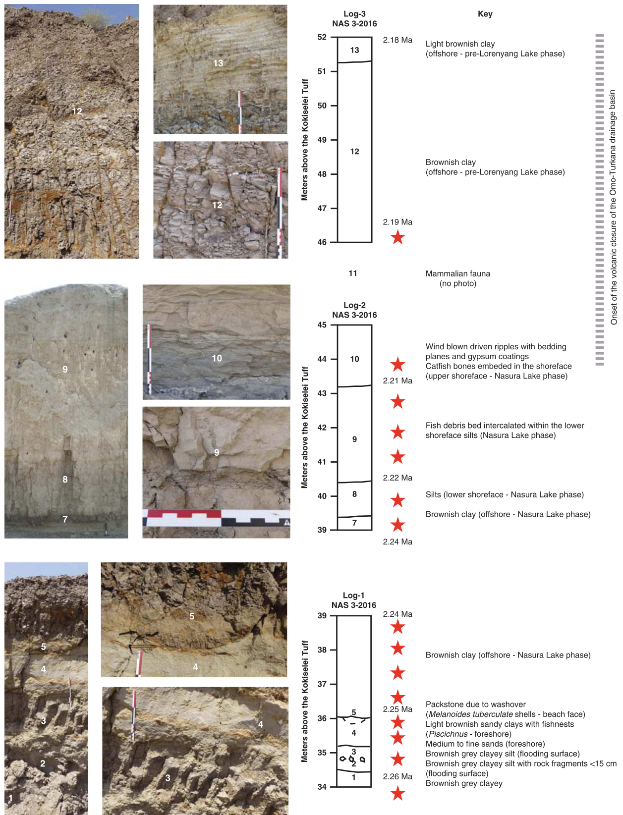
Figure 5. Lithology and stratigraphy of the Nasura Lake phase (Nasura locality). The red stars represent the analyzed geochemical samples. See Figure 2 for the location of the examined outcrops. (For interpretation of the references to color in this figure legend, the reader is referred to the web version of this article.)
