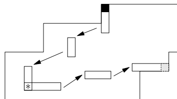
Figure 2: The path of the \square in a local evacuation-shuffle. The black and gray squares are the initial and final locations of the \square ; the algorithm switched from “Phase 1” to “Phase 2” at the square marked by a *. There is an antidiagonal symmetry : the Phase 1 path forms a vertical strip, while the Phase 2 path forms a horizontal strip. We give a precise statement of this symmetry in the full paper.
