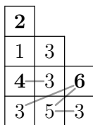
Fig. 1: A filling of a Young diagram. Descents are shown in bold, and attacking pairs are connected by a segment.
