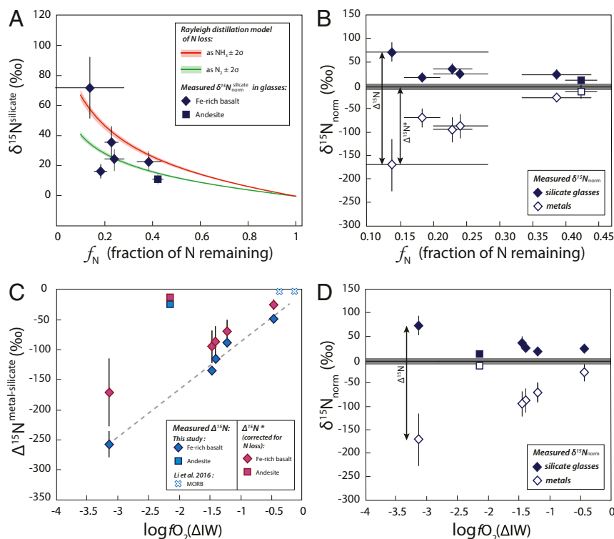
Fig. 3. Effect of N loss (A and B) and f_{O_2} (C and D) on N-isotopic fractionation \Delta^{15}N^{\text{metal-silicate}} . (A) Modeled effect of N loss by Rayleigh distillation on the \delta^{15}N_{\text{norm}} values of silicate glasses as a function of f_N , the fraction of N remaining in the sample at the end of the experiments compared with the initial N content of the starting materials. The \delta^{15}N_{\text{silicate}} values represent measured ^{15}N/^{14}N_{\text{silicate}} ratios normalized to the initial ^{15}N/^{14}N ratio of the starting material (see text and Table 1). Rayleigh distillation was modeled for N_2 loss (green curve) and NH_3 loss (red curve) as \delta^{15}N_{\text{silicate}} = 1,000 \cdot (f_N^{(1/\alpha)} - 1) , where \alpha is the fractionation factor approximated here by \sqrt{[m(^{15}N) + m(^{14}N)]/m(^{14}N_2)} = 1.02 for N_2 loss and by \sqrt{[m(^{15}N) + 3 \cdot m(H)]/[m(^{14}N) + 3 \cdot m(H)]} = 1.03 for NH_3 loss. The positive \delta^{15}N values measured in our silicate glasses can be explained by the Rayleigh distillation model, suggesting that N loss may have increased the \delta^{15}N values of the silicate glasses. (B) Evolution of \delta^{15}N in the silicate glasses (closed symbols) and in the metal blobs (open symbols) as a function of f_N . The \delta^{15}N_{\text{norm}} values represent measured ^{15}N/^{14}N^p ratios ( p representing the metallic or silicate phase) normalized to the initial ^{15}N/^{14}N ratio of the starting material (see text and Table 1), and the gray line at 0‰ represents the initial \delta^{15}N_{\text{norm}} value. The difference between the \delta^{15}N values measured in the metal and the silicate phases ( \delta^{15}N_{\text{metal}} - \delta^{15}N_{\text{silicate}} ) approximates the calculated \Delta^{15}N^{\text{metal-silicate}} values. Considering that positive \delta^{15}N_{\text{norm}} values may have been produced by N loss, the difference between the initial \delta^{15}N_{\text{norm}} (0‰) and the \delta^{15}N_{\text{norm}} values corresponds to \Delta^{15}N^* , the N-isotopic fractionation corrected for N loss. (C) \Delta^{15}N^{\text{metal-silicate}} as a function of f_{O_2} , showing both calculated \Delta^{15}N^{\text{metal-silicate}} (blue symbols) and \Delta^{15}N^* (purple symbols). The small blue x's are reproduced from Li et al. (16), with f_{O_2} values recalculated following the procedure described in the text. Error bars represent 2\sigma SDs. Whereas the uncertainties on \Delta^{15}N^{\text{metal-silicate}} are determined from the SDs on ^{15}N/^{14}N ratios measured by SIMS, the larger uncertainties on f_N , \delta^{15}N_{\text{norm}} values, and \Delta^{15}N^* are derived from the weighing uncertainties associated with the addition of Si_3^{14}N_4 and Si_3^{15}N_4 to the starting materials. The dashed line represents a linear regression ( r^2 > 0.9 ) on the \Delta^{15}N^{\text{metal-silicate}} values measured in Fe-rich basalt. \Delta^{15}N^{\text{metal-silicate}} data describe 2 trends that can be explained by compositionally dependent differences in N speciation in the silicate glasses (see text). (D) Evolution of \delta^{15}N_{\text{norm}} in the silicate glasses and metal blobs as a function of f_{O_2} . This plot shows that positive \delta^{15}N_{\text{norm}} values can also be produced by N-isotopic fractionation during metal segregation from the melt via the formation of ^{14}N -Fe bonds in the metal from ^{14}N in NH complexes in the melt. This process becomes more important as the f_{O_2} decreases due to the increasing stabilization of NH complexes in the melt under more reducing conditions.
