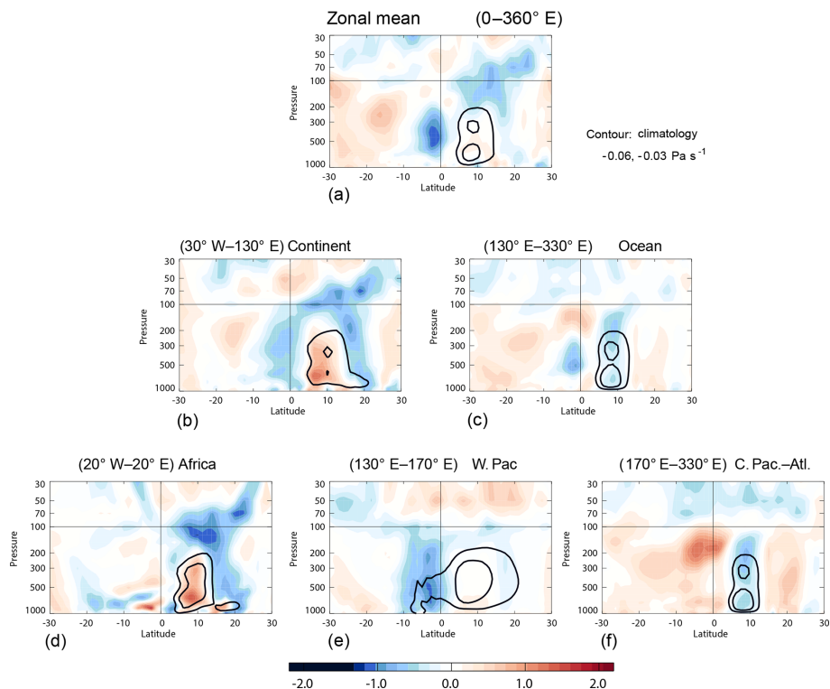
Figure 7. (a) Standardized anomalous pressure vertical velocity (departures from 1981–2010 climatology) – the climatological JAS mean zonal-mean pressure vertical velocity is indicated by contours ( -0.06 and -0.03 \text{ Pa s}^{-1} ); (middle panels) same as (a) but for (b) the African–Asian continental sector ( 30^\circ \text{ W} – 130^\circ \text{ E} ) and (c) the Pacific–Atlantic oceanic sector ( 130^\circ \text{ E} – 330^\circ \text{ E} ); (bottom panels) same as (a) but for (d) the African continental sector ( 20^\circ \text{ W} – 20^\circ \text{ E} ), (e) the western Pacific sector ( 130^\circ \text{ E} – 170^\circ \text{ E} ), and (f) the central Pacific–Atlantic sector ( 170^\circ \text{ E} – 330^\circ \text{ E} ).
