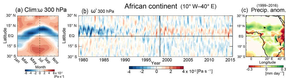
Figure 5. (a) Latitude–time section of the climatological zonal-mean pressure vertical velocity at 300 hPa averaged over the African sector (10° W–40° E), (b) latitude–time section of monthly mean anomalous pressure vertical velocity from February 1979 to November 2016, and (c) latitude–longitude map of annual mean anomalous precipitation during 1999–2016 over the African sector. A 3-month running mean is applied in (b).
