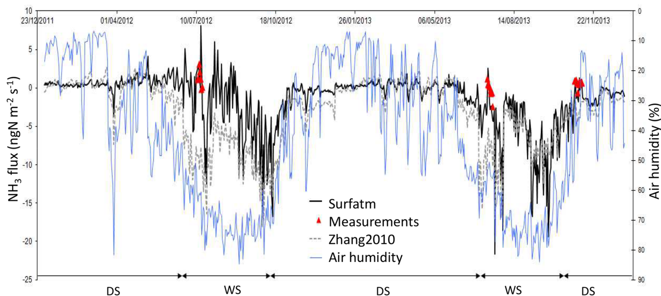
Figure 9. Daily \text{NH}_3 flux ( \text{ngN m}^{-2} \text{s}^{-1} ) simulated by Surfalm (black line) and Zhang2010 (grey dashed line) and daily averaged \text{NH}_3 flux measurements during three field campaigns (red triangles). Error bars in red stand for standard deviation at the daily scale. Air humidity as a percentage (blue line). DS: dry season; WS: wet season.
