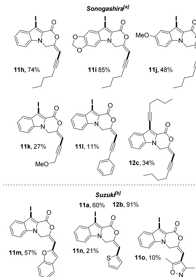
Scheme 10. Structures and yields of the Sonogashira and Suzuki couplings.
