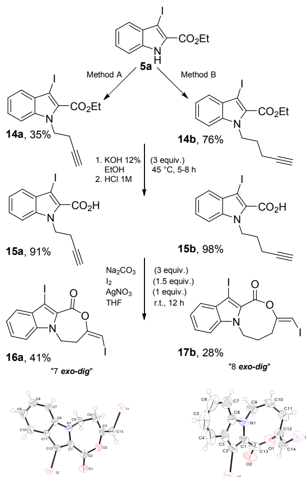
Scheme 12. Extended alkynyl chain indoles and X-Ray structures of compounds 16a and 17b with displacement ellipsoids.
