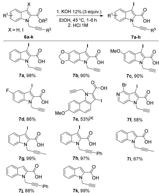
Scheme 5. Scope of the saponification step.
