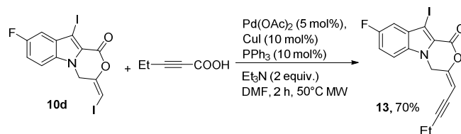
Scheme 11. Sonogashira decarboxylative cross-coupling reaction with 10d .
