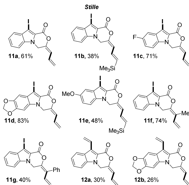
Scheme 9. Structures and yields of the Stille coupling. Reagents and conditions: vinyltin (1.1 equiv.), PdCl 2 MeCN 2 (5 mol%), DMF, r.t., 18 h.
