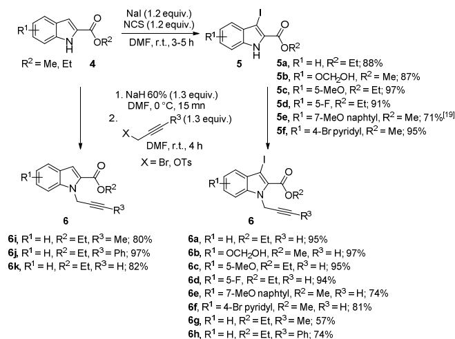
Scheme 2. Precursor preparation.
