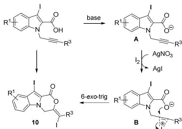
Scheme 7. Proposed mechanism for iodolactonization.
