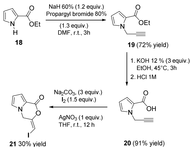
Scheme 13. Pyrrole extension.
