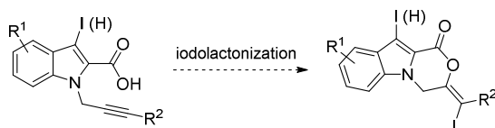
Scheme 1. Synthesis of indoles fused at 2,3 and 1,2.
