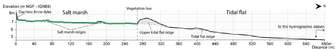
Figure 2. Schematic topographic profile, Western part of the Bay of Mont-Saint-Michel.
