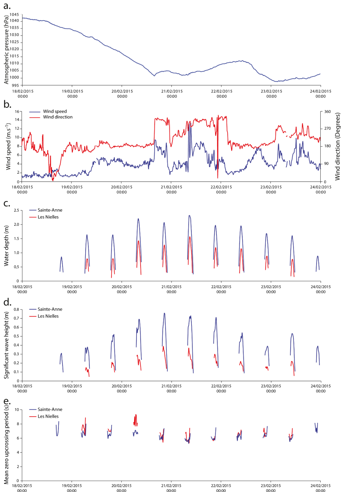
Figure 5. Synthesis of hydrodynamics data during Experiment 1 - February 2015 - (a) atmospheric pressure data, (b) wind data, (c) water depth data, (d) significant wave height data, (e) mean zero upcrossing period data.
