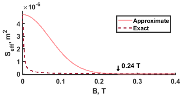
FIG. 7. Comparison of the approximate and exact theories for r_{pr} = 75 \mu m. The arrow indicates the intersection.
