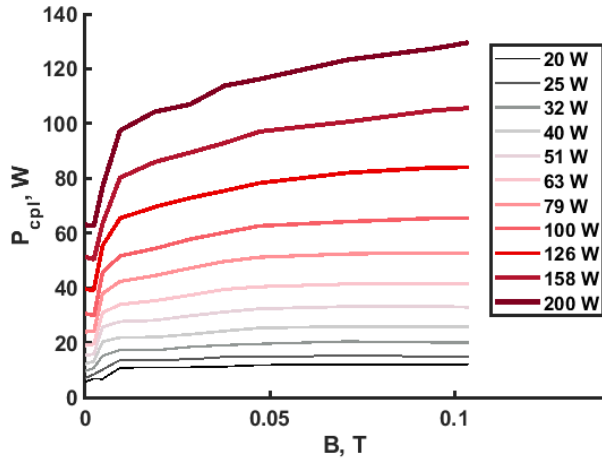
FIG. 5. Variation of the coupled power for various forward power.
