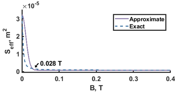
FIG. 8. Comparison of the approximate and exact theories for r_{pr} = 0.5 mm. The arrow indicates the intersection.
