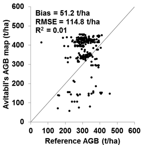
Fig. 12. Avitabile's AGB map against the reference AGB maps of the four Gabonese regions.
