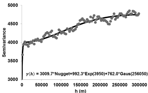
Fig. 8. Semivariogram of the residuals. Nugget = 3009 (t/ha) 2 .
